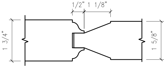
PANEL A1 (RIM BANDED)
