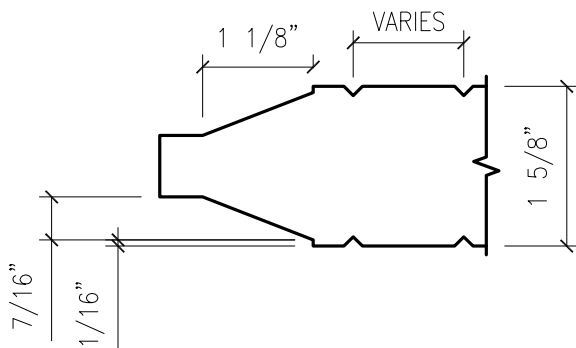
V-GROOVE RAISED PANEL (RIM BANDED)
