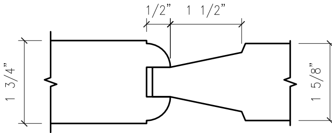
PANEL 3 (RIM BANDED)
