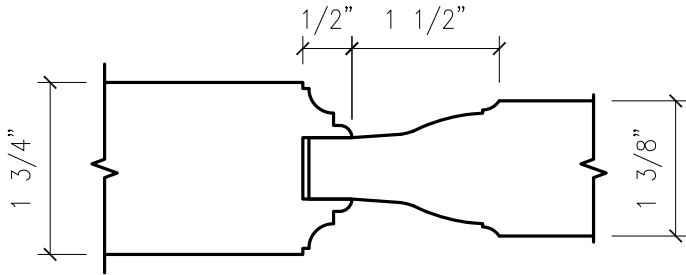
PANEL R1 (RIM BANDED)
