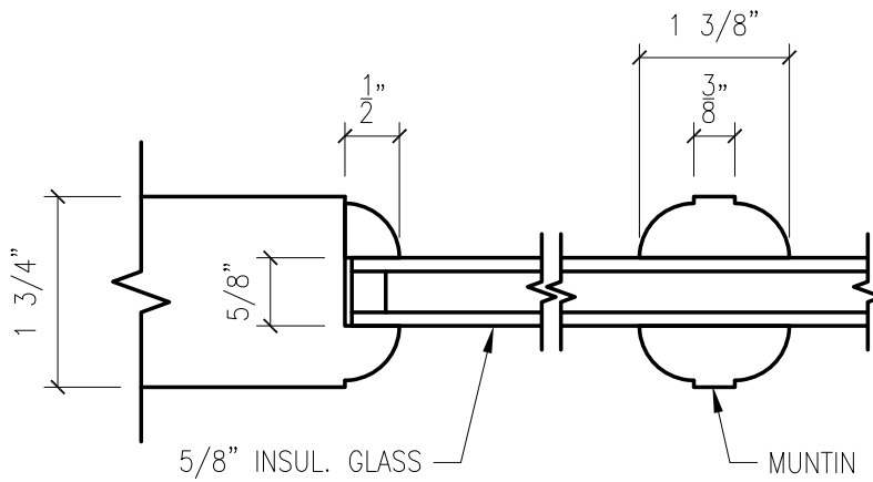
STANDARD SIMULATED DIVIDED LITE (SDL)
