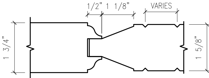
V-GROOVE RAISED PANEL
