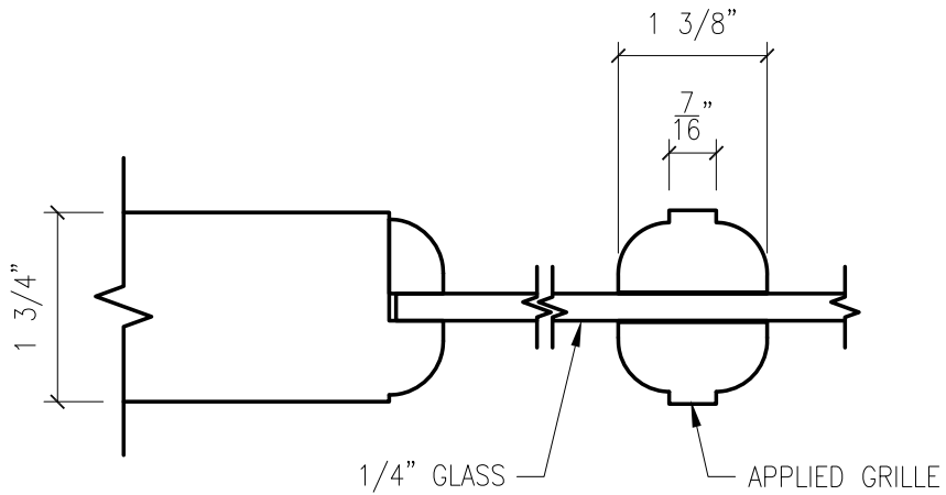
STANDARD SIMULATED DIVIDED LITE (SDL)
