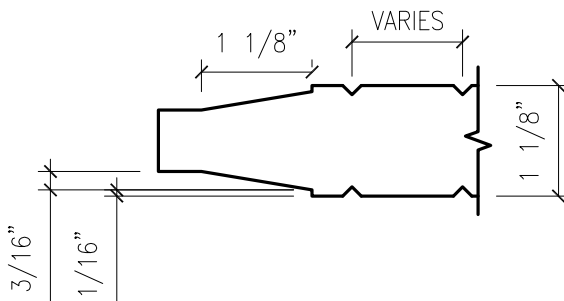
V-GROOVE RAISED PANEL (RIM BANDED)
