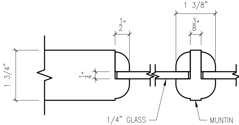
STANDARD TRUE DIVIDED LITE (TDL)
